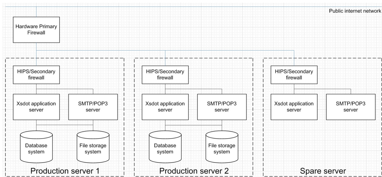
ASP Hardware/Software Hosting cluster
